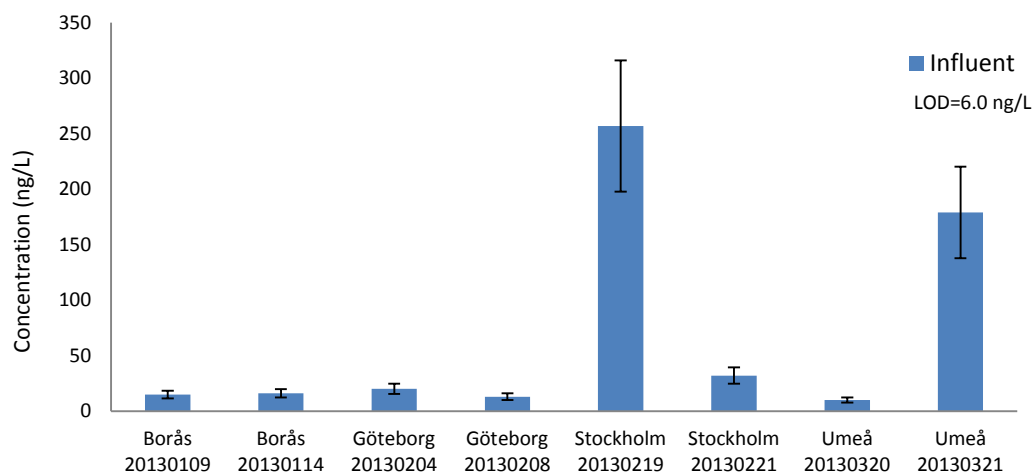
Figure 3. Concentration of the sum of ZnPT and CuPT in influent waste water from the four sewage treatment plants in the national programme, each sampled at two occasions. The concentration in the corresponding effluent waters were <6 ng/L in all cases. Error bars represent the relative standard deviation (RSD) established for the method (Table 7).
